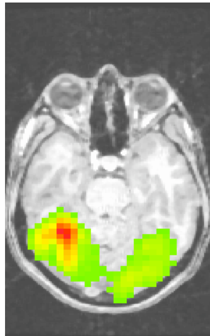
3dmerge -1filter_aver 8
