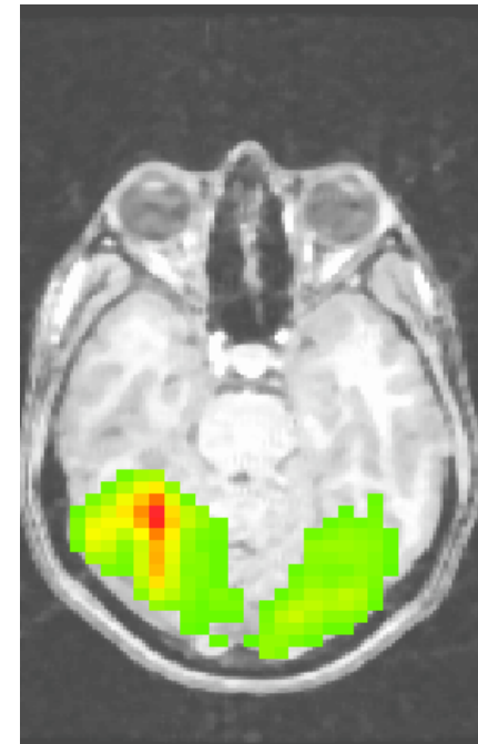
3dmerge -1blur_fwhm 8
